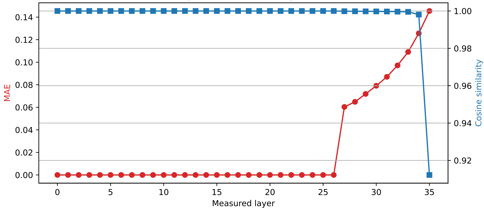
SmolLM3-3B | Quantized layer 26 | float32 \rightarrow int2
