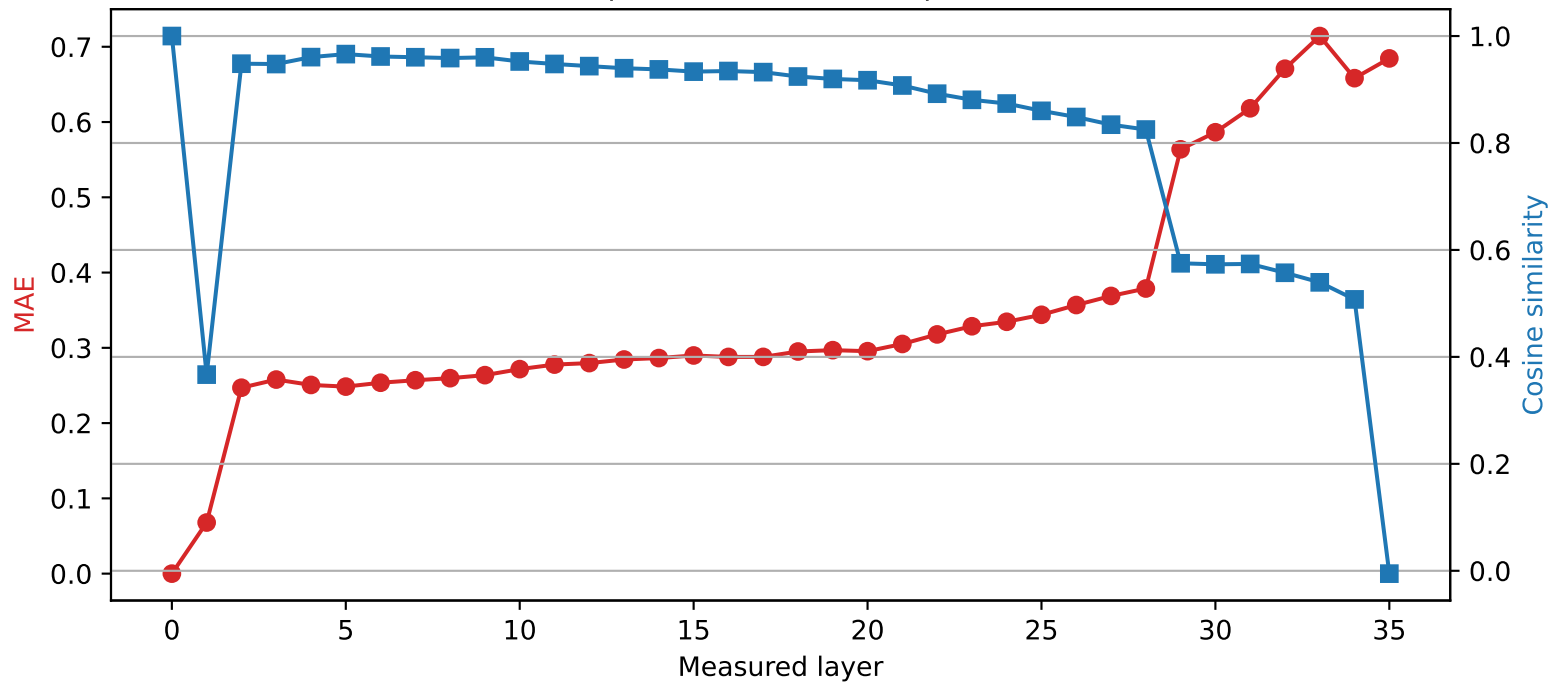
SmolLM3-3B | Quantized layer 0 | float32 \rightarrow int2
