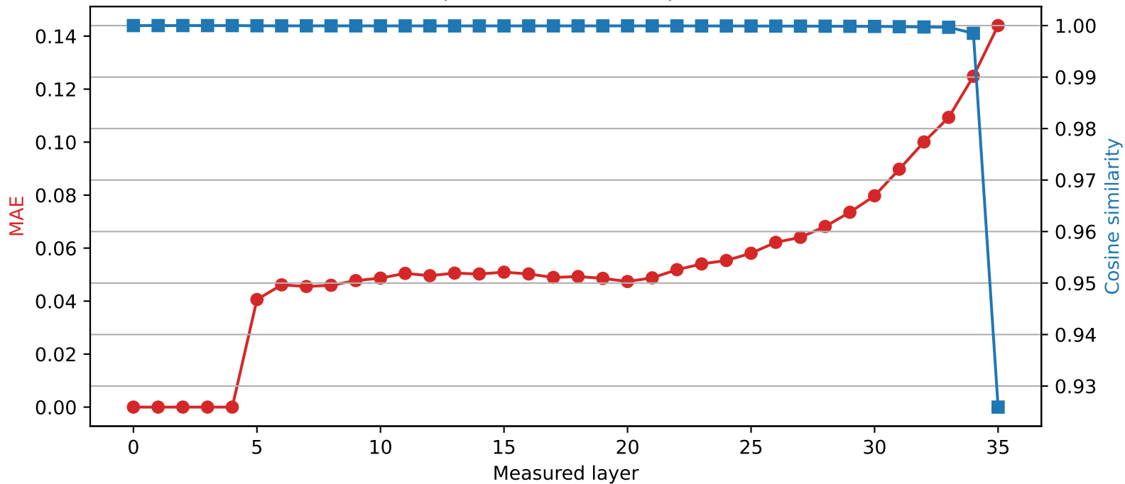
SmolLM3-3B | Quantized layer 4 | float32 \rightarrow int2
