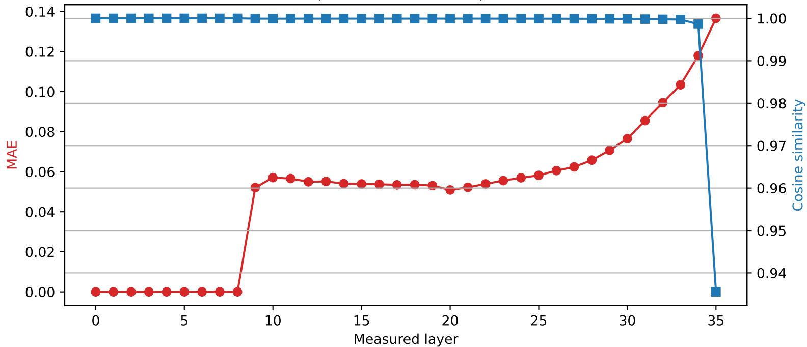
SmolLM3-3B | Quantized layer 8 | float32 \rightarrow int2
