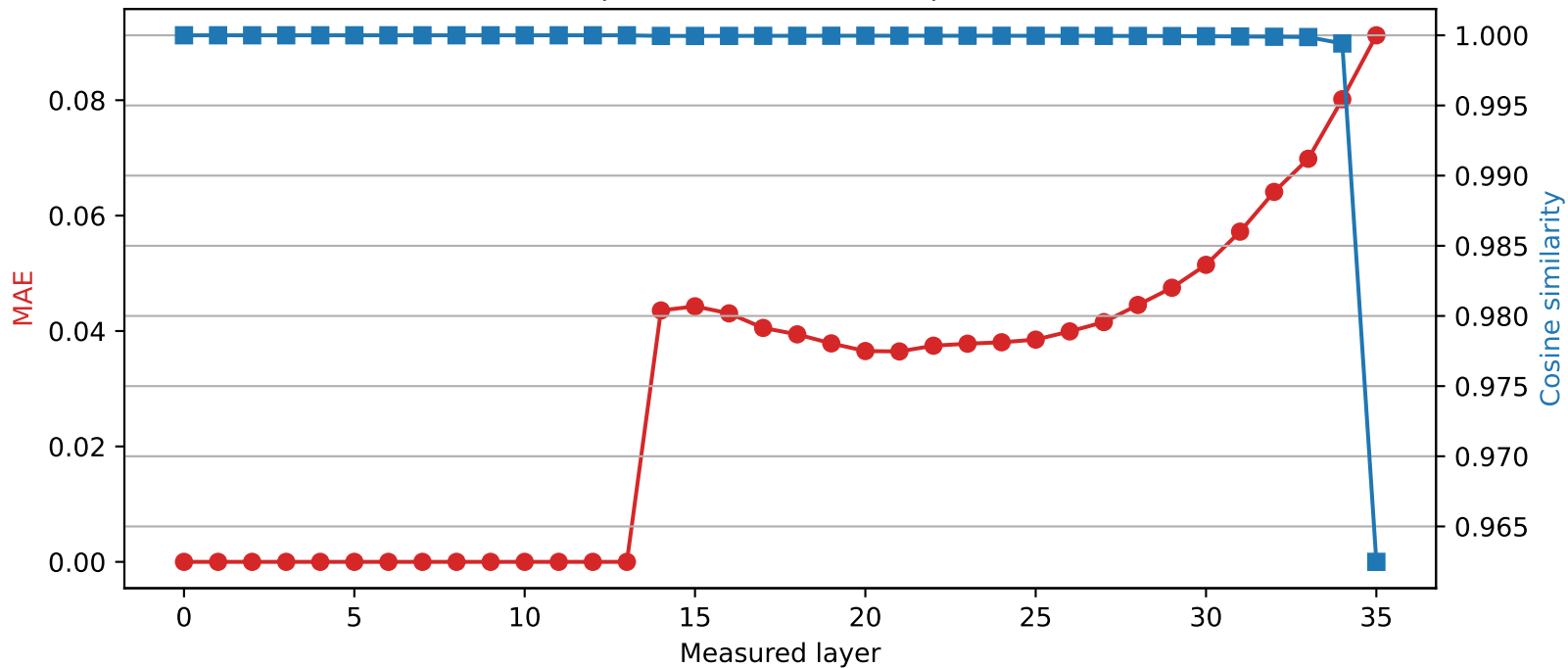
SmolLM3-3B | Quantized layer 13 | float32 → int2
