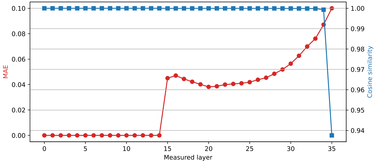
SmolLM3-3B | Quantized layer 14 | float32 → int2
