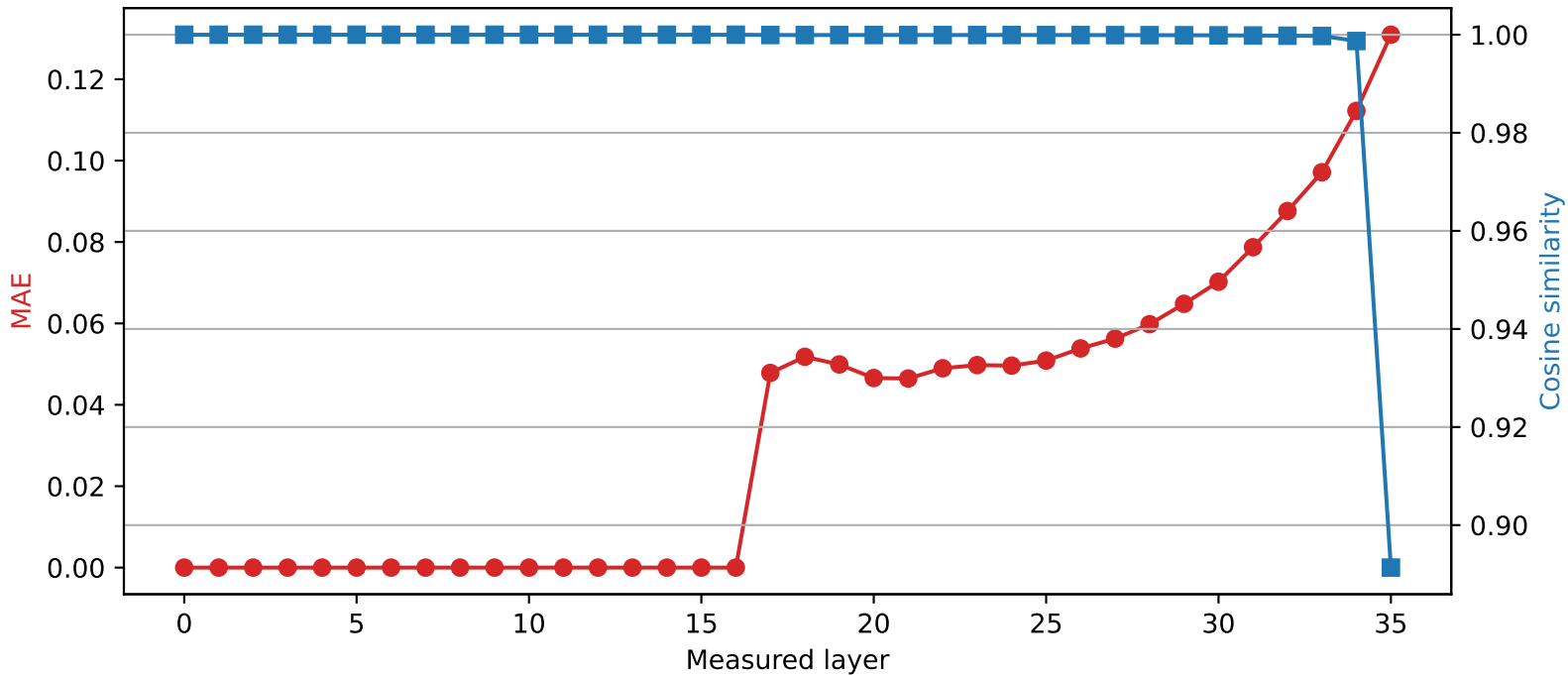
SmolLM3-3B | Quantized layer 16 | float32 → int2
