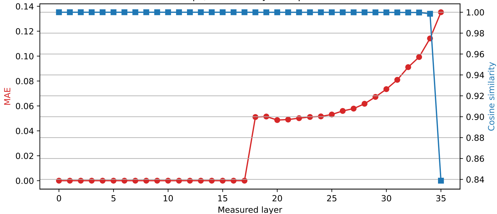
SmolLM3-3B | Quantized layer 17 | float32 → int2
