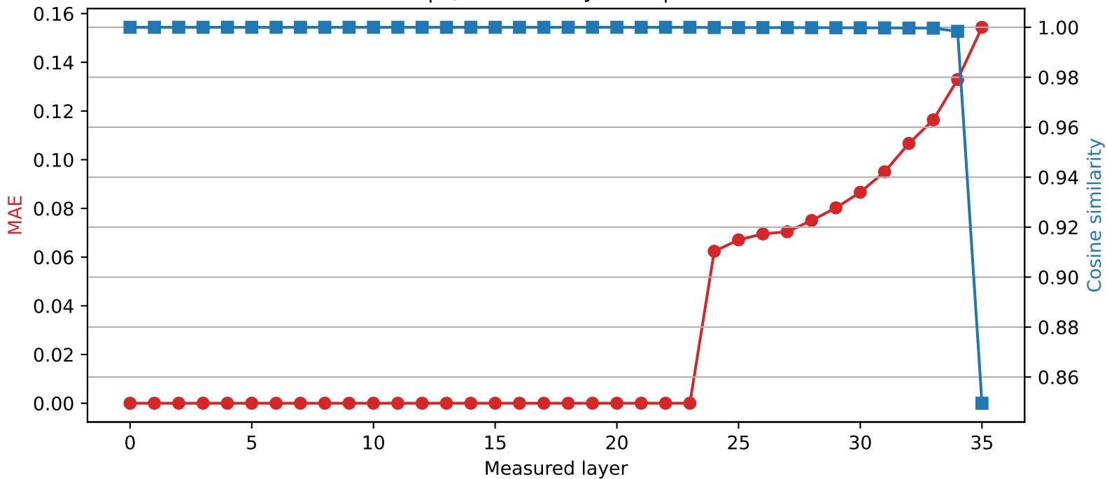
SmolLM3-3B | Quantized layer 23 | float32 \rightarrow int2
