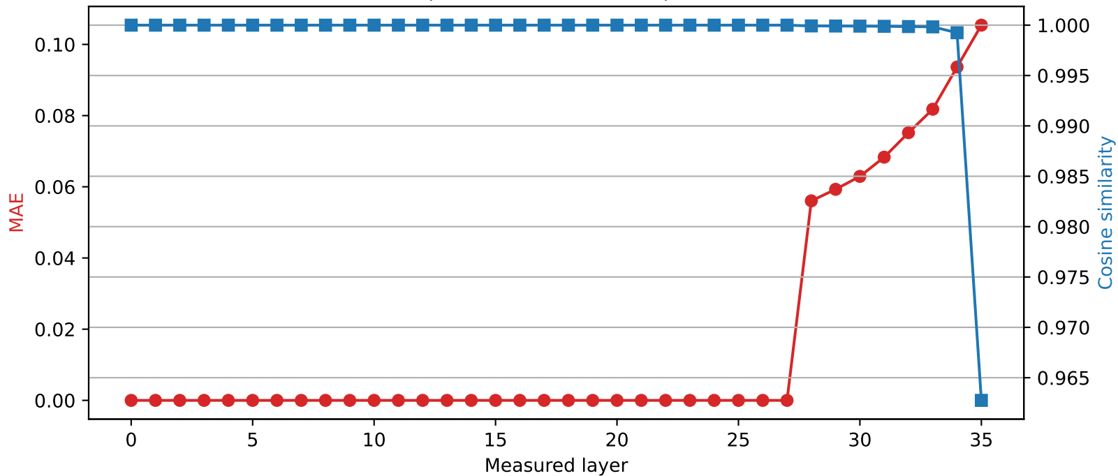
SmolLM3-3B | Quantized layer 27 | float32 \rightarrow int2
