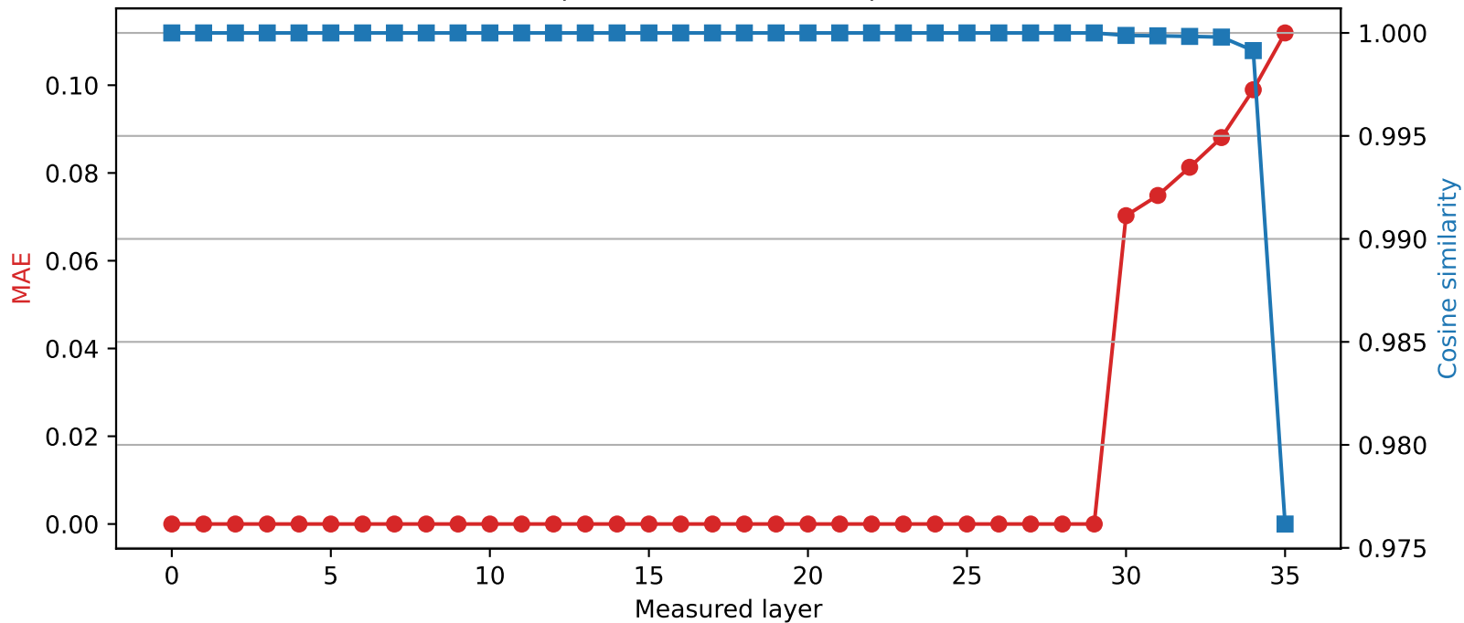
SmolLM3-3B | Quantized layer 29 | float32 \rightarrow int2
