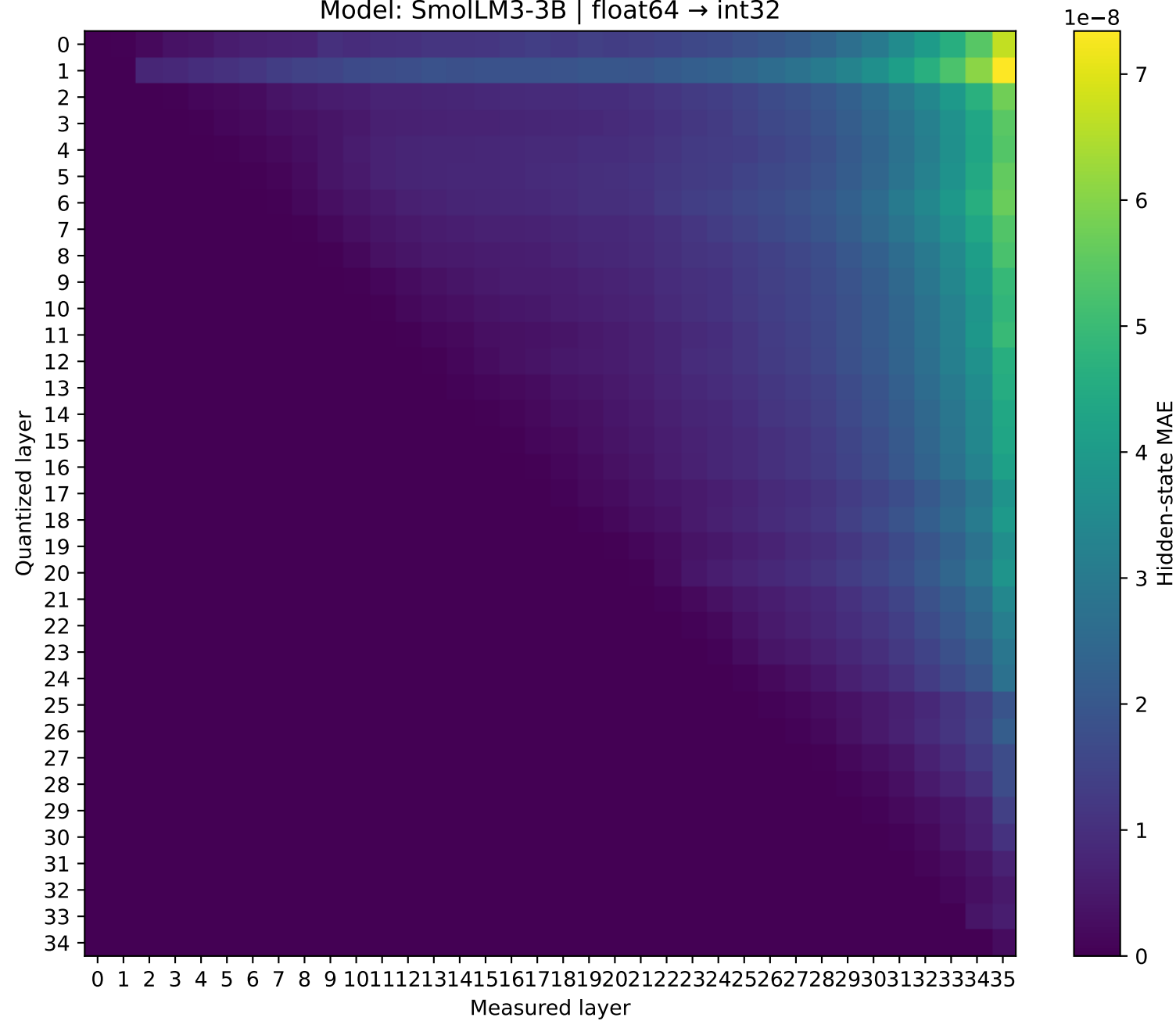
Model: SmolLM3-3B | float64 \rightarrow int32
