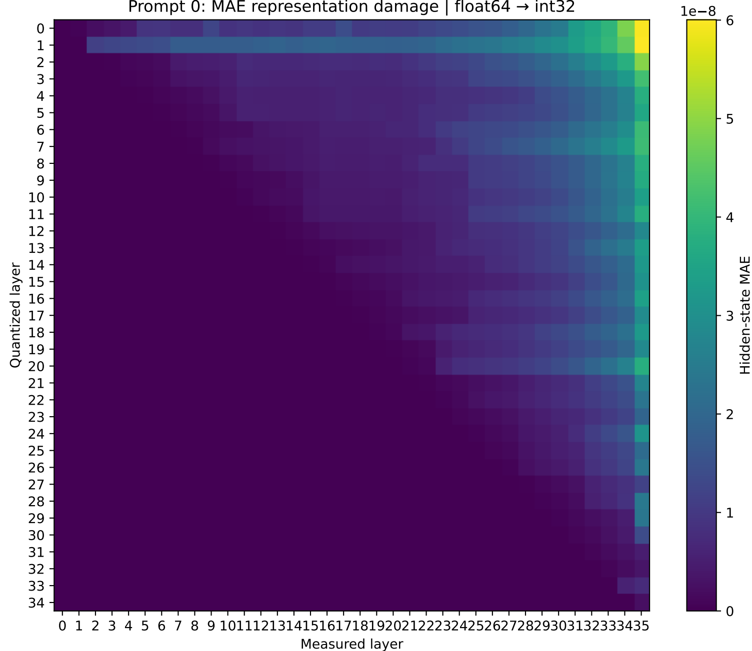
SmolLM3-3B Prompt 0: MAE representation damage | float64 → int32
