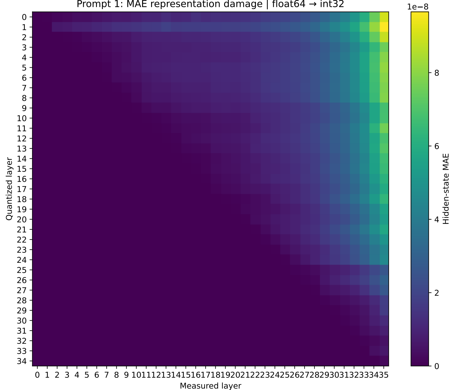
SmolLM3-3B Prompt 1: MAE representation damage | float64 → int32
