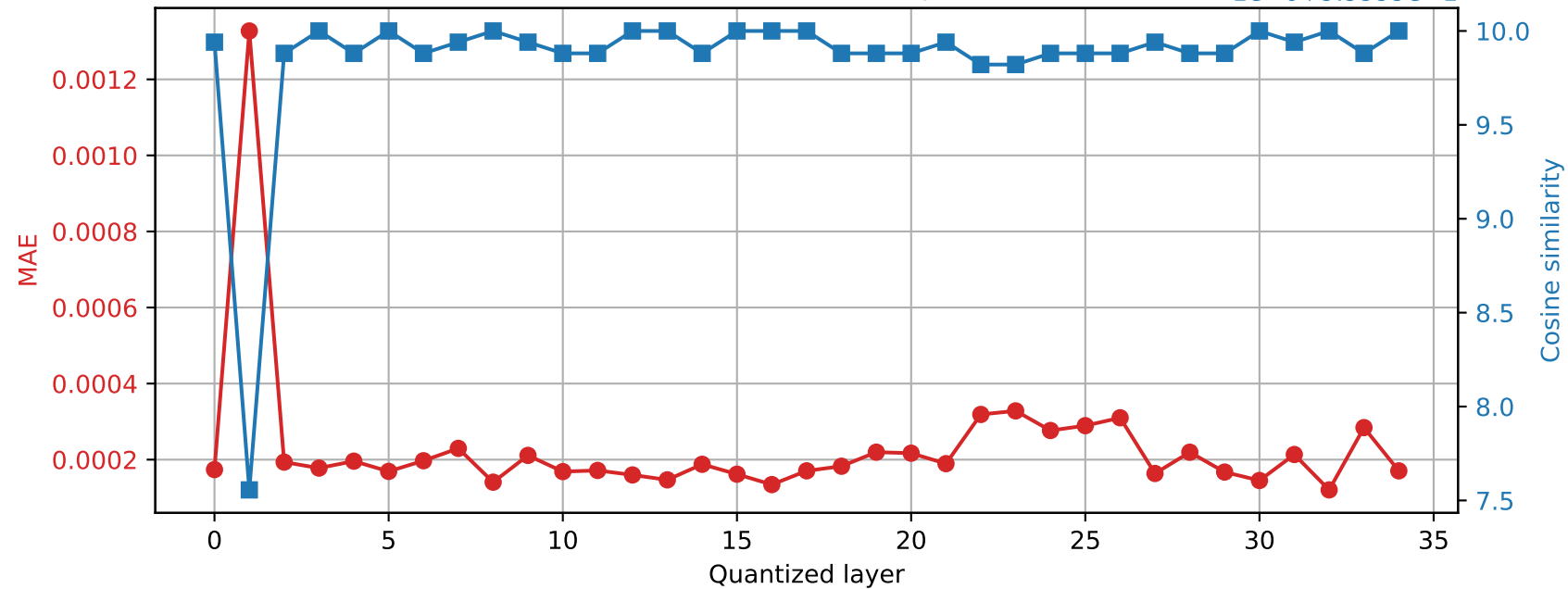
SmolLM3-3B | Prompt 1 Final RMSNorm output damage | float64 → int16
