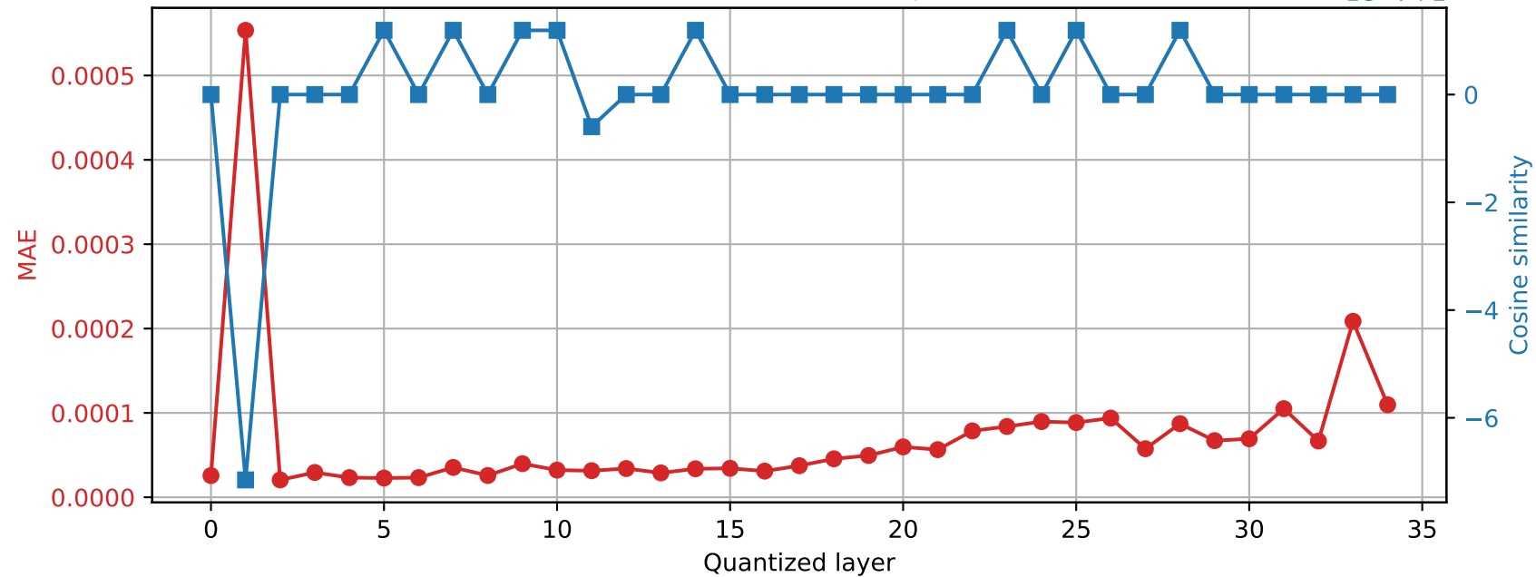
SmolLM3-3B | Prompt 2 Final RMSNorm output damage | float64 → int16
