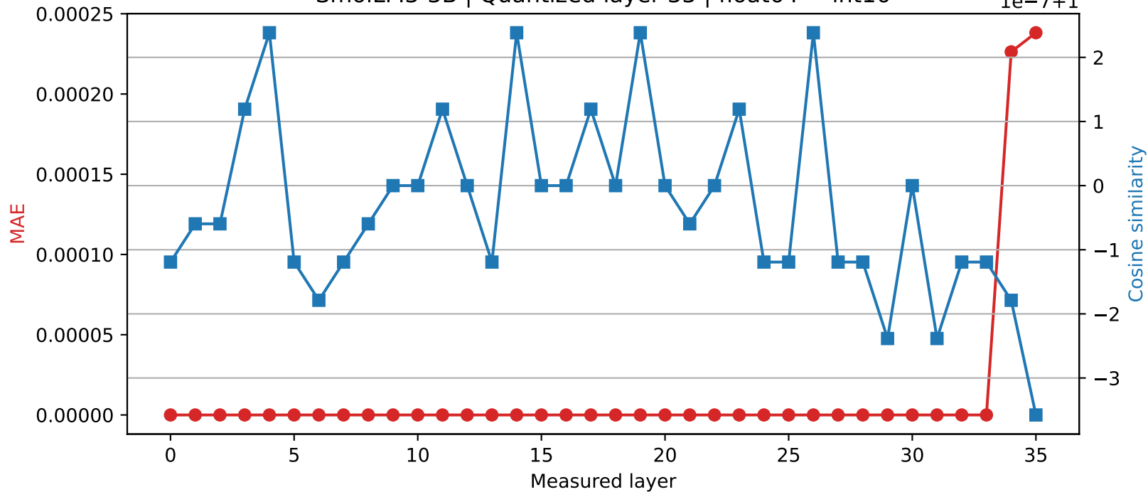
SmolLM3-3B | Quantized layer 33 | float64 \rightarrow int16
