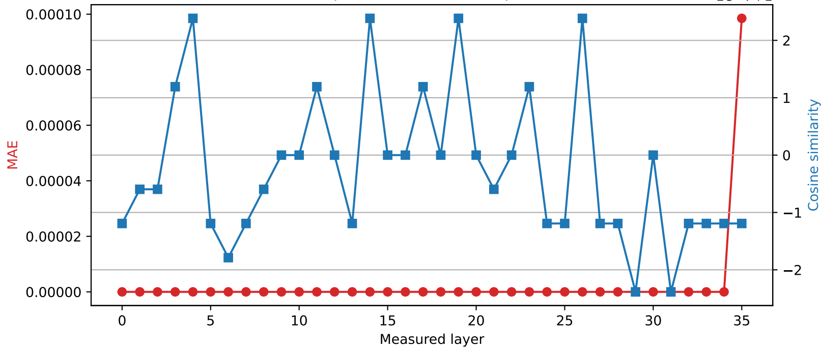
SmolLM3-3B | Quantized layer 34 | float64 → int16
