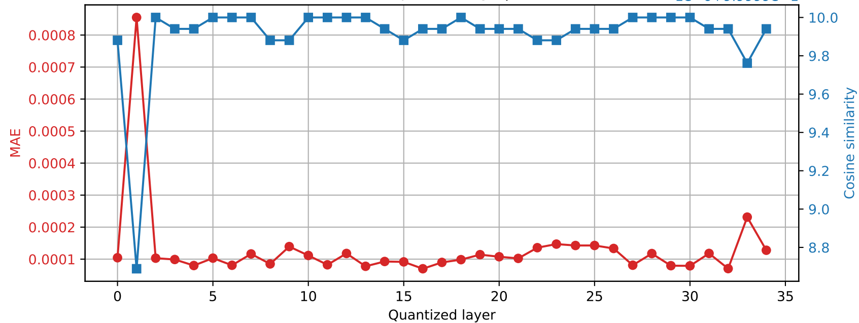
SmolLM3-3B | Prompt 3 Final RMSNorm output damage | float64 → int16
