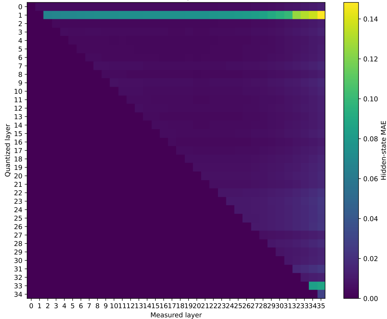
Model: SmolLM3-3B | float64 → int8
