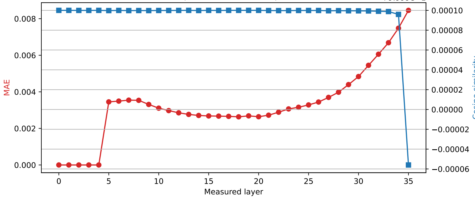
SmolLM3-3B | Quantized layer 4 | float64 → int8
