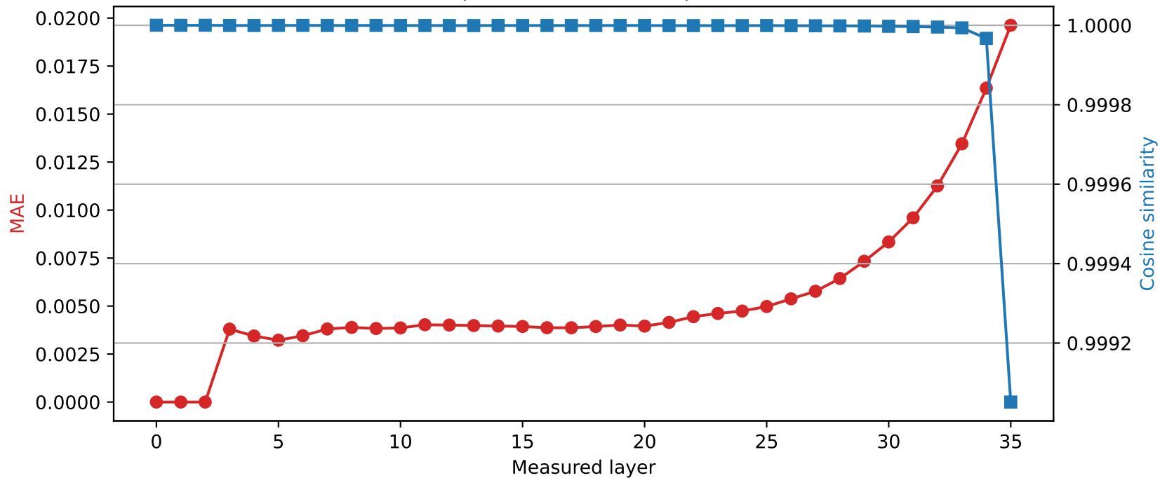
SmolLM3-3B | Quantized layer 2 | float64 \rightarrow int8
