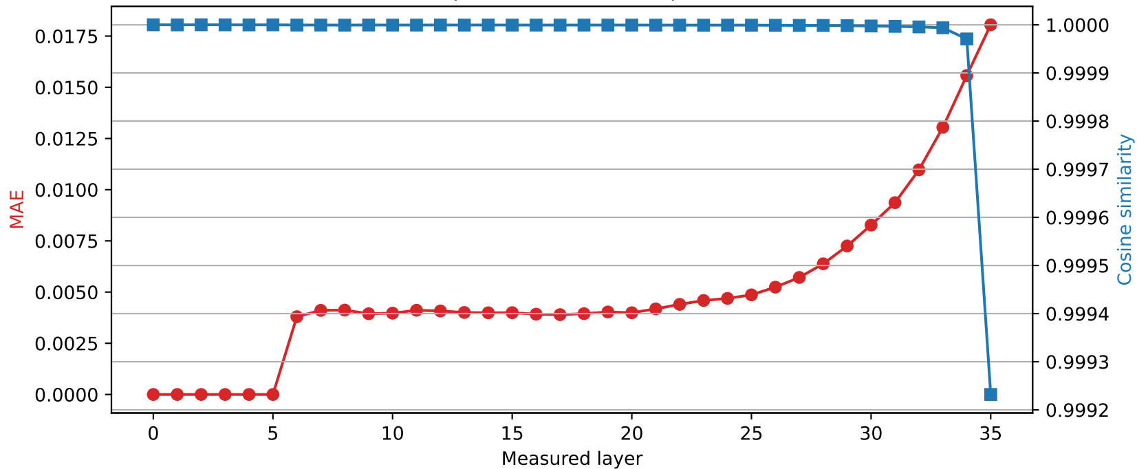
SmolLM3-3B | Quantized layer 5 | float64 → int8
