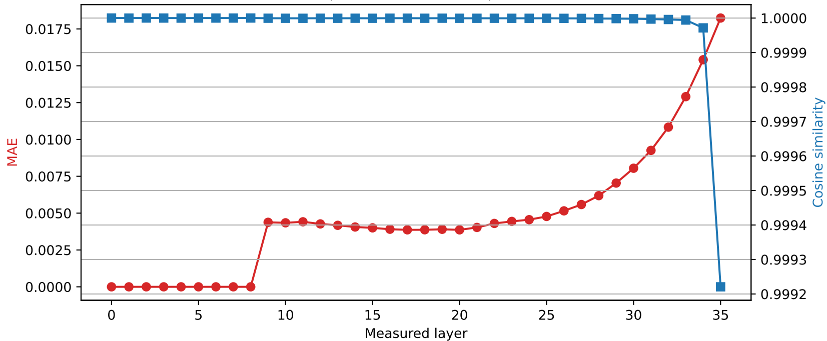
SmolLM3-3B | Quantized layer 8 | float64 \rightarrow int8
