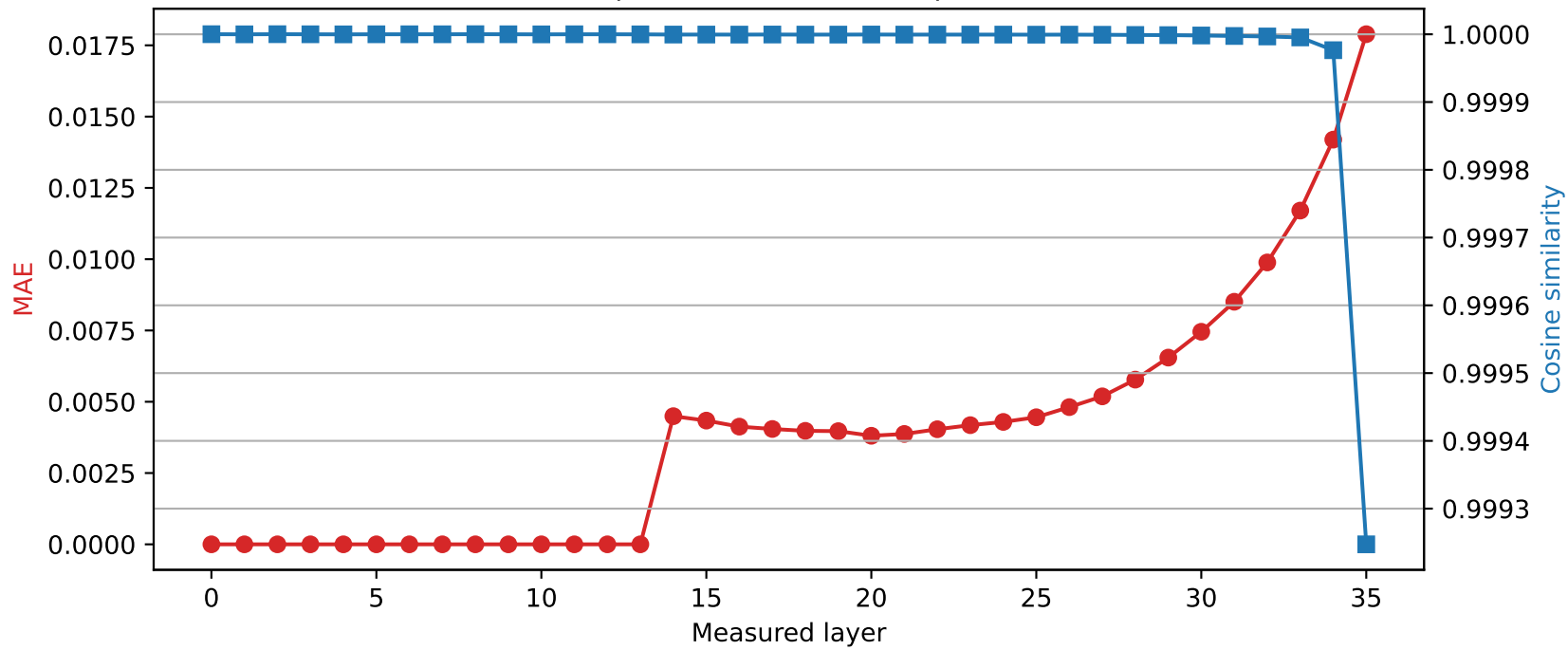
SmolLM3-3B | Quantized layer 13 | float64 → int8
