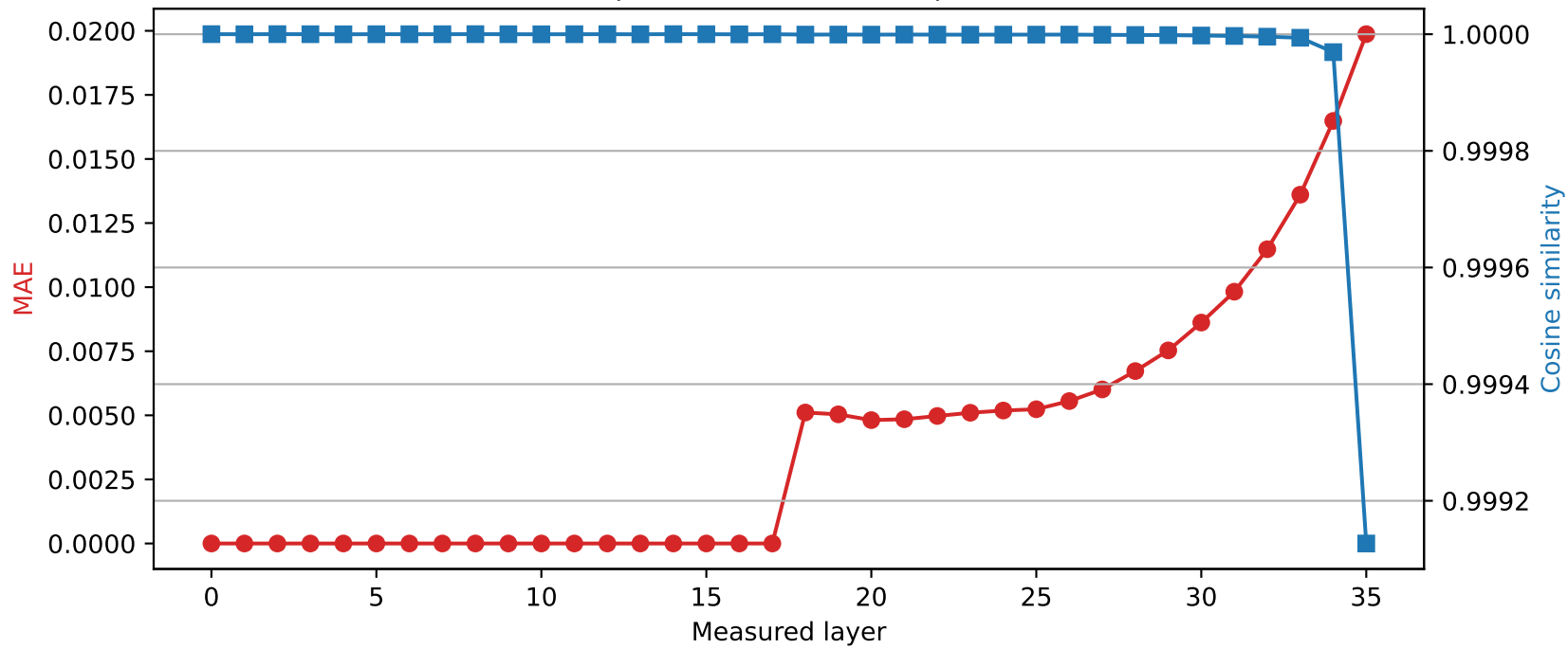
SmolLM3-3B | Quantized layer 17 | float64 → int8
