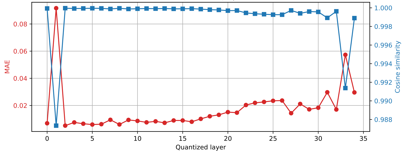
SmolLM3-3B | Prompt 2 Final RMSNorm output damage | float64 → int8
