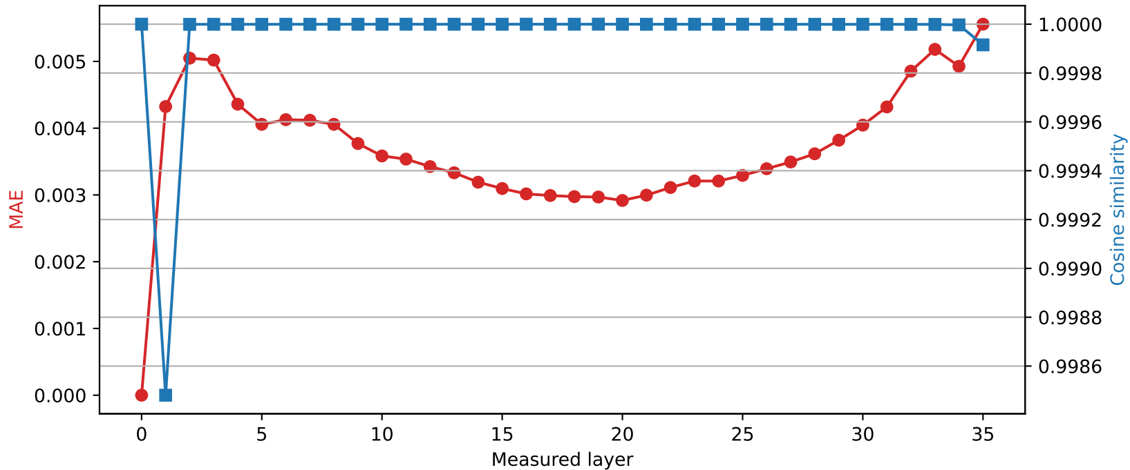
SmolLM3-3B | Quantized layer 0 | float64 → int8
