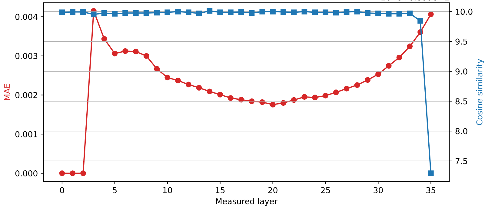
SmolLM3-3B | Quantized layer 2 | float64 → int8
