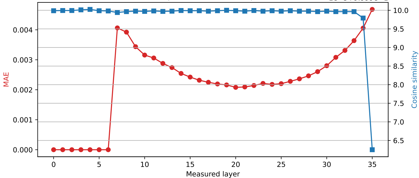
SmolLM3-3B | Quantized layer 6 | float64 → int8
