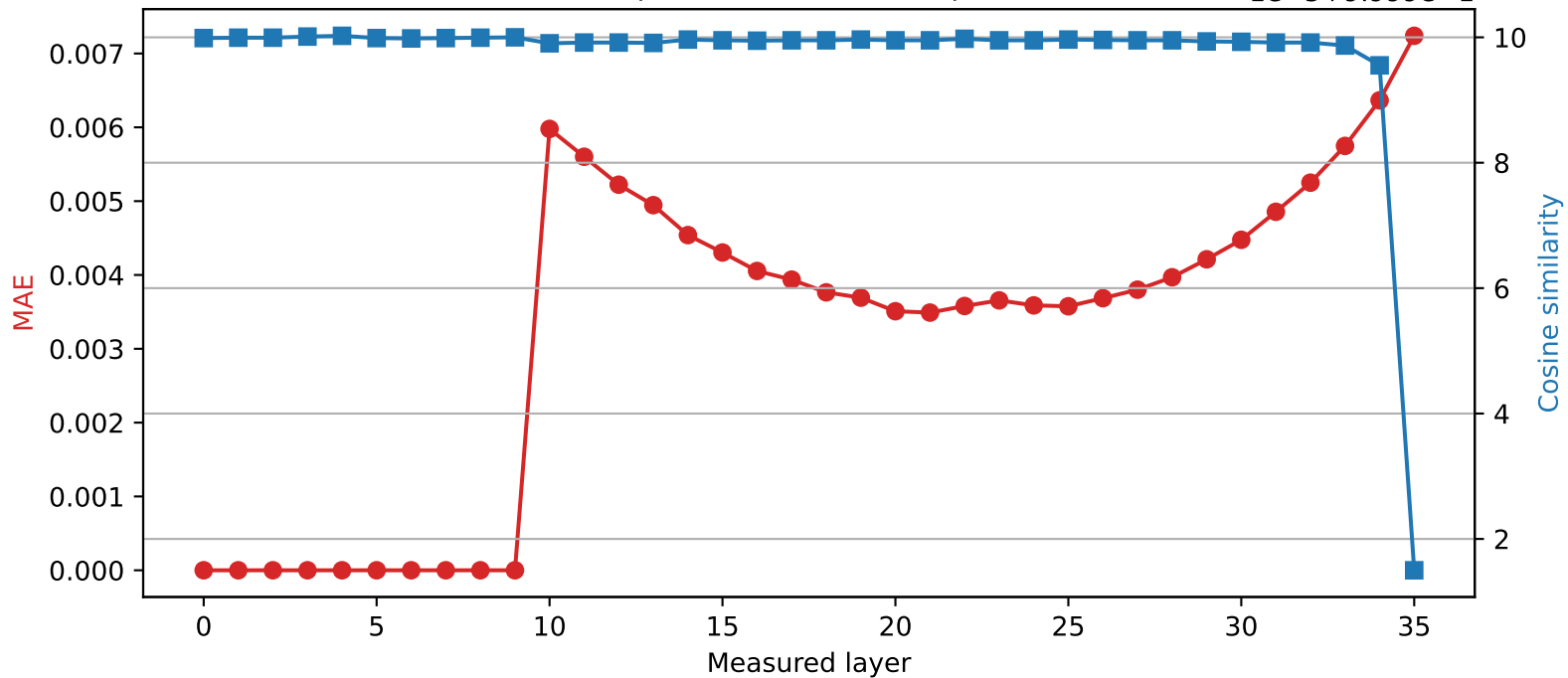
SmolLM3-3B | Quantized layer 9 | float64 → int8
