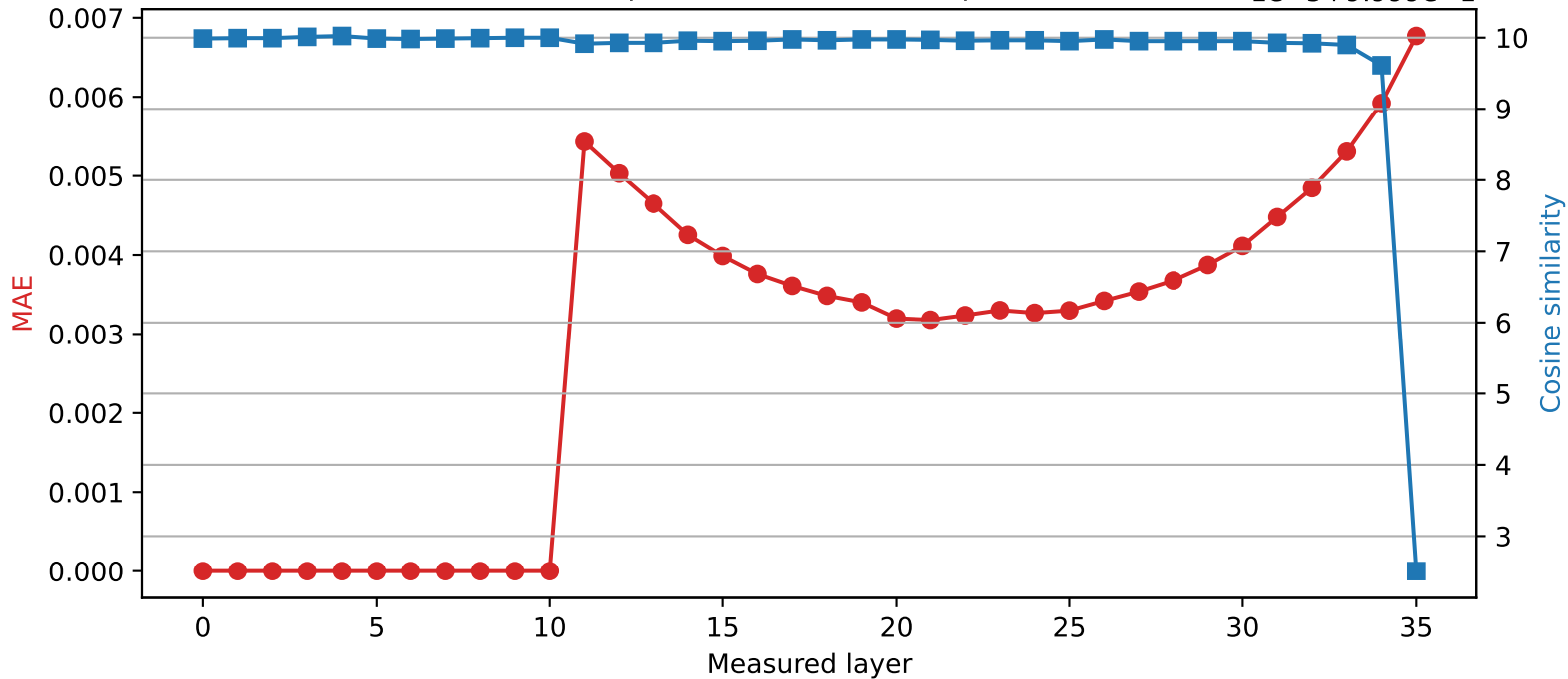
SmolLM3-3B | Quantized layer 10 | float64 → int8
