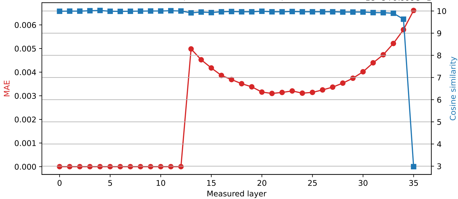
SmolLM3-3B | Quantized layer 12 | float64 → int8
