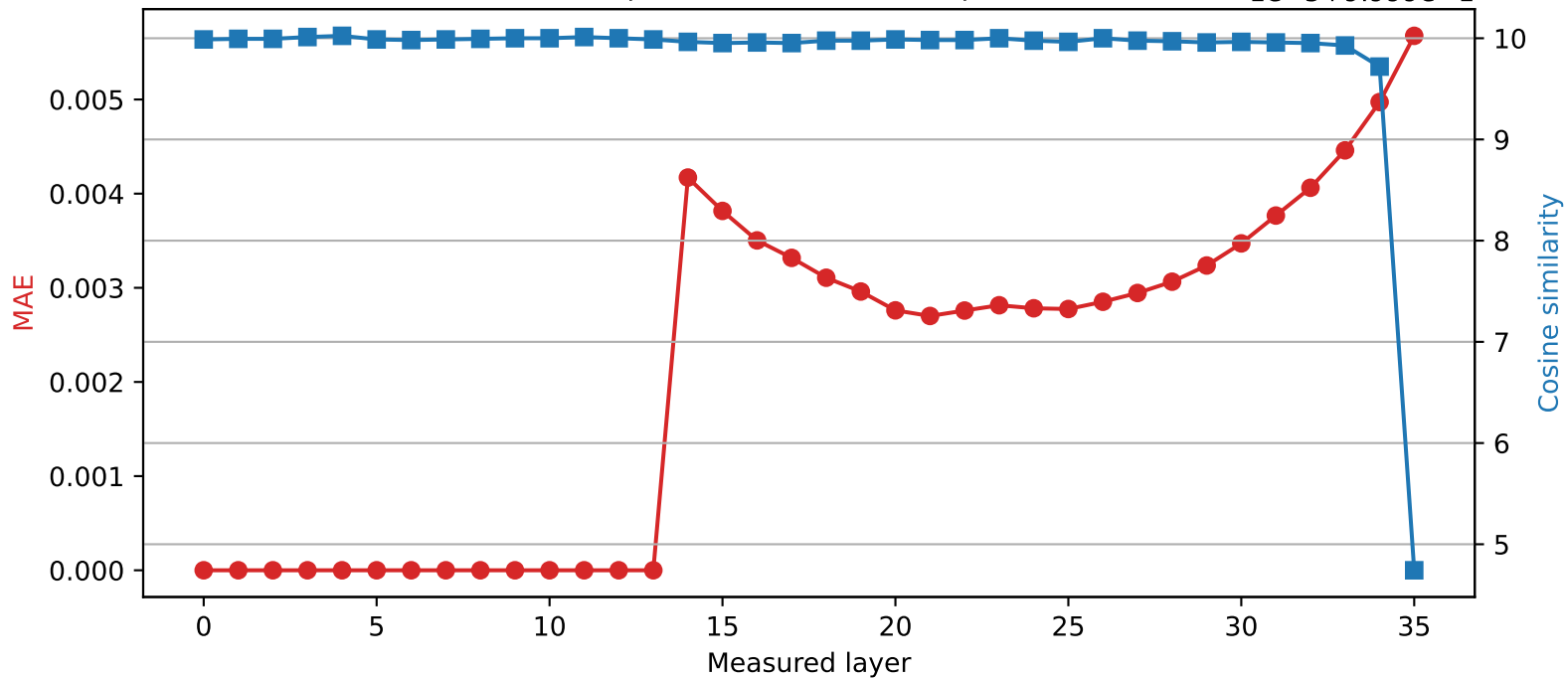
SmolLM3-3B | Quantized layer 13 | float64 → int8
