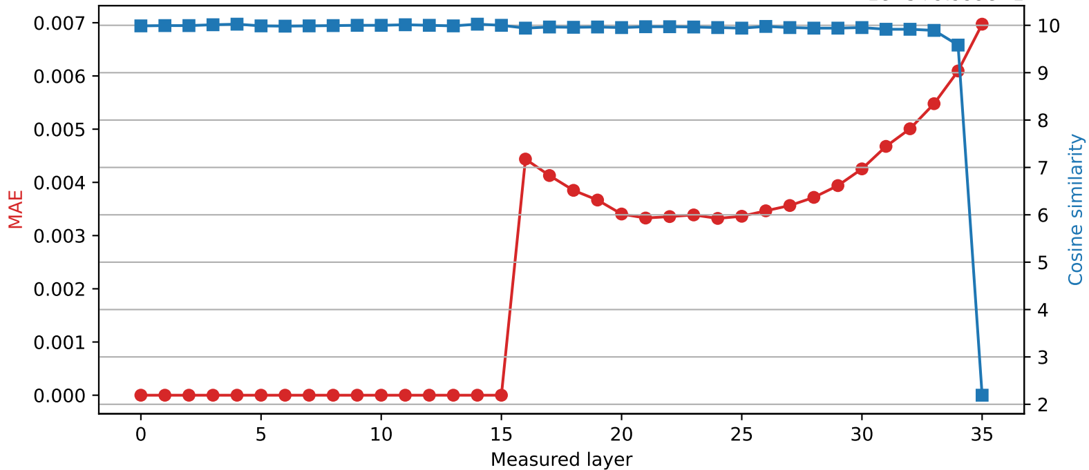
SmolLM3-3B | Quantized layer 15 | float64 → int8
