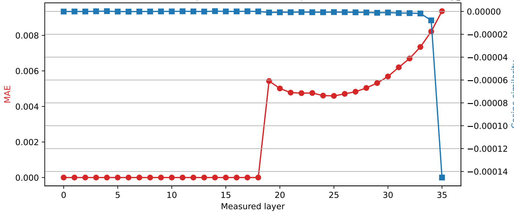
SmolLM3-3B | Quantized layer 18 | float64 → int8
