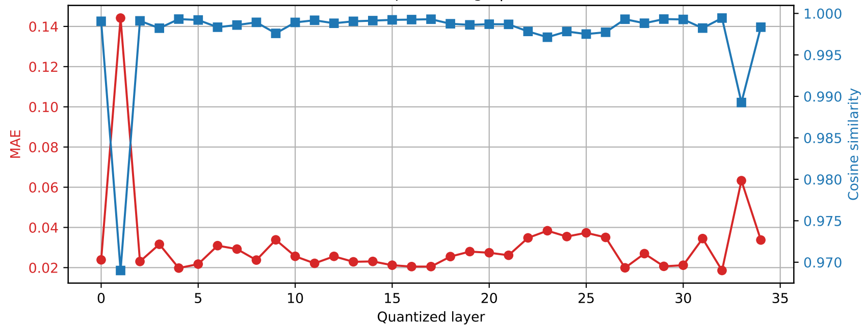
SmolLM3-3B | Prompt 3 Final RMSNorm output damage | float64 \rightarrow int8
