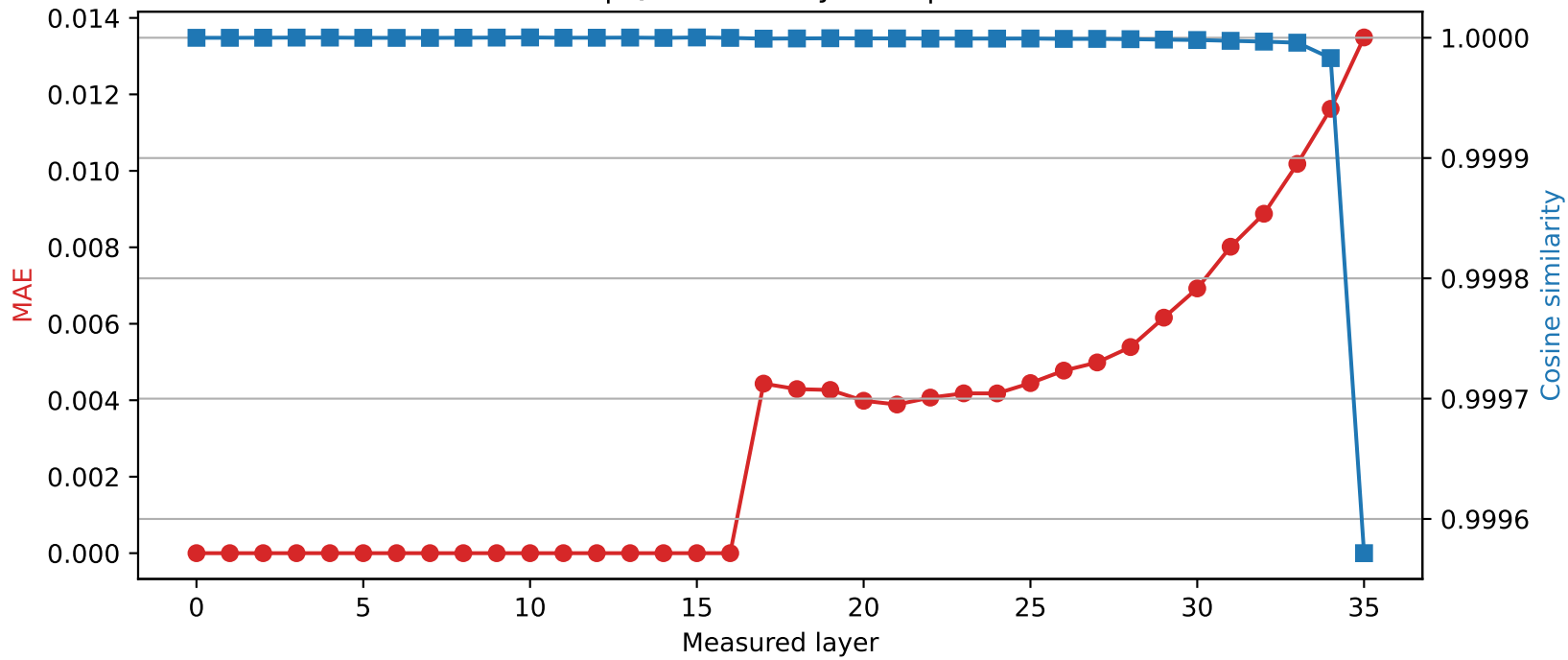
SmolLM3-3B | Quantized layer 16 | float64 → int8
