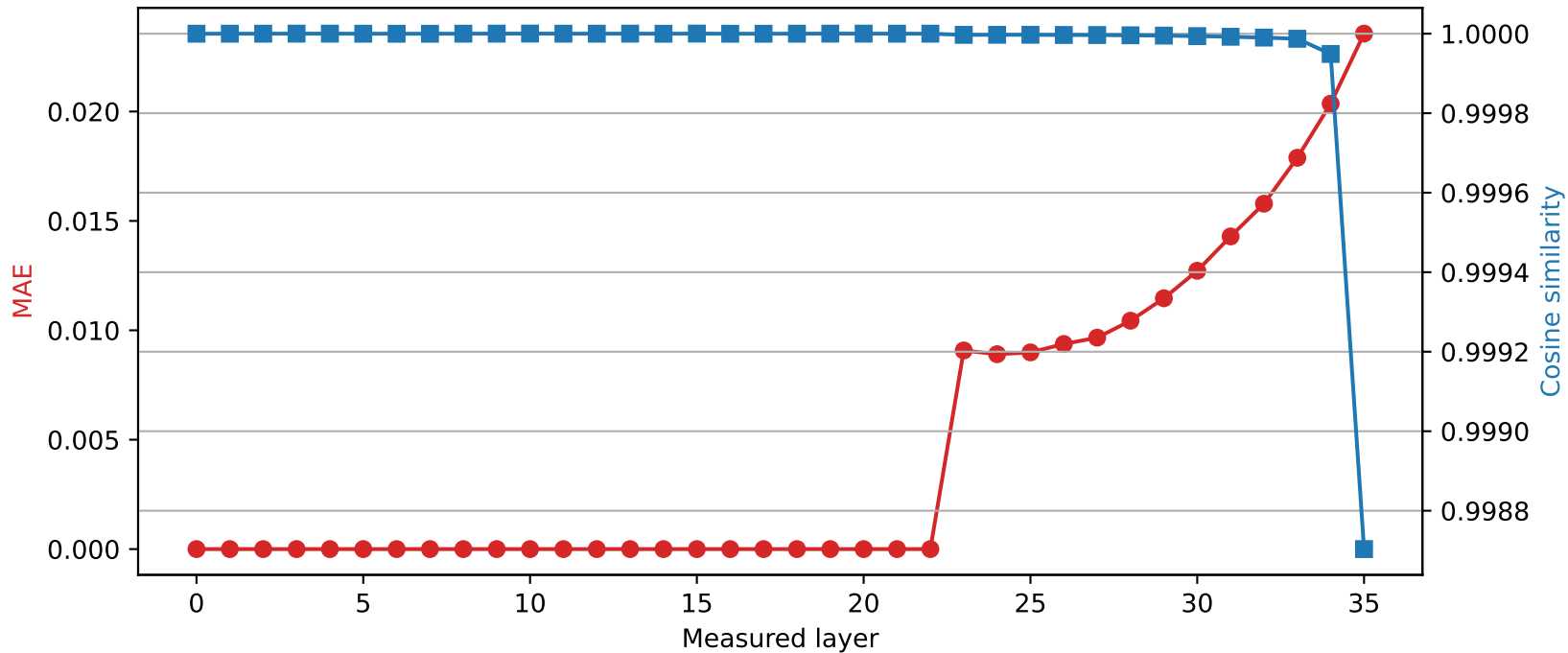
SmolLM3-3B | Quantized layer 22 | float64 → int8
