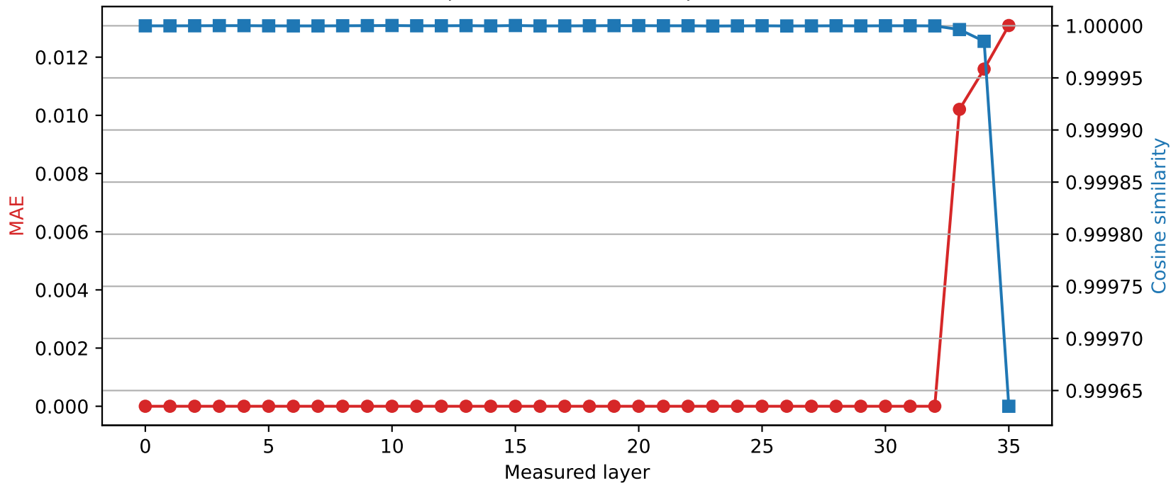
SmolLM3-3B | Quantized layer 32 | float64 → int8
