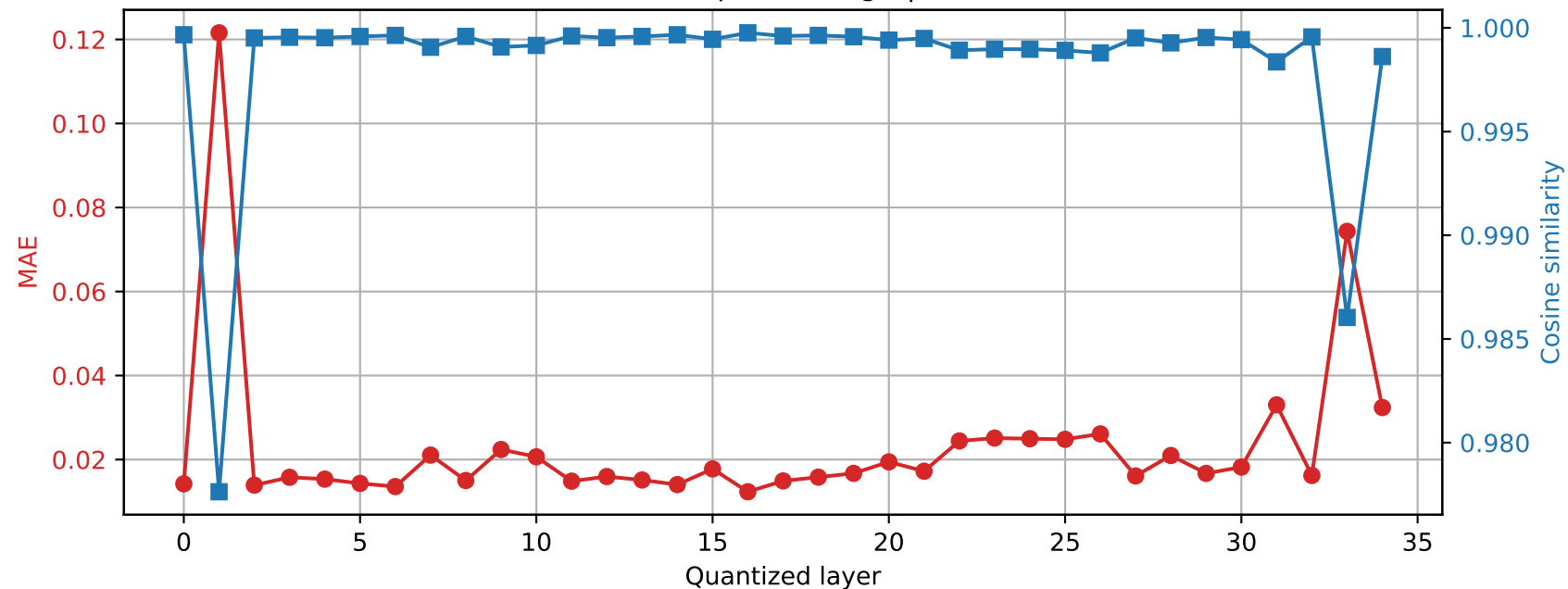
SmolLM3-3B | Prompt 4 Final RMSNorm output damage | float64 → int8
