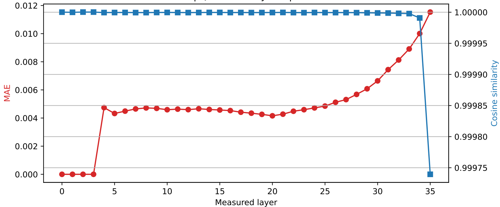
SmolLM3-3B | Quantized layer 3 | float64 → int8
