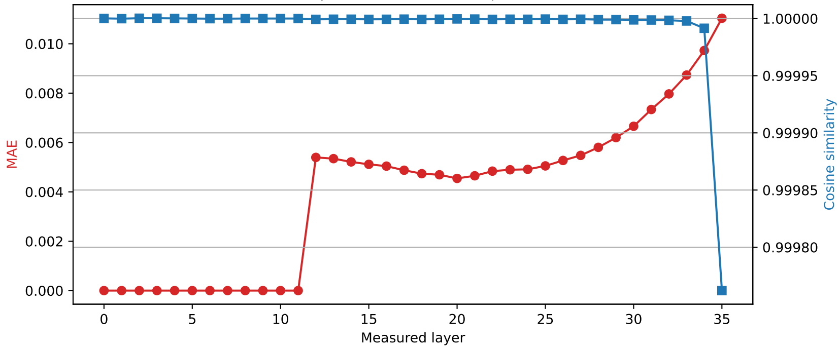
SmolLM3-3B | Quantized layer 11 | float64 → int8
