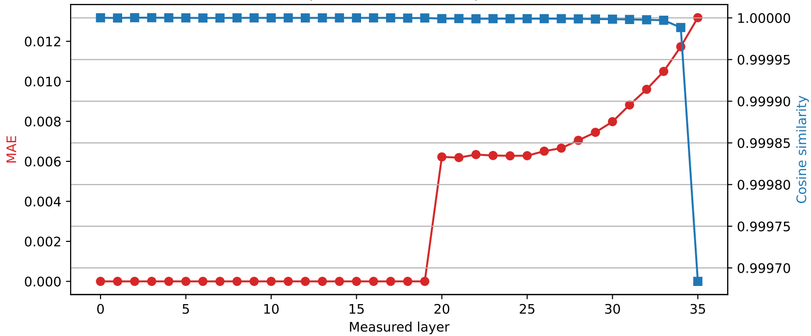
SmolLM3-3B | Quantized layer 19 | float64 → int8
