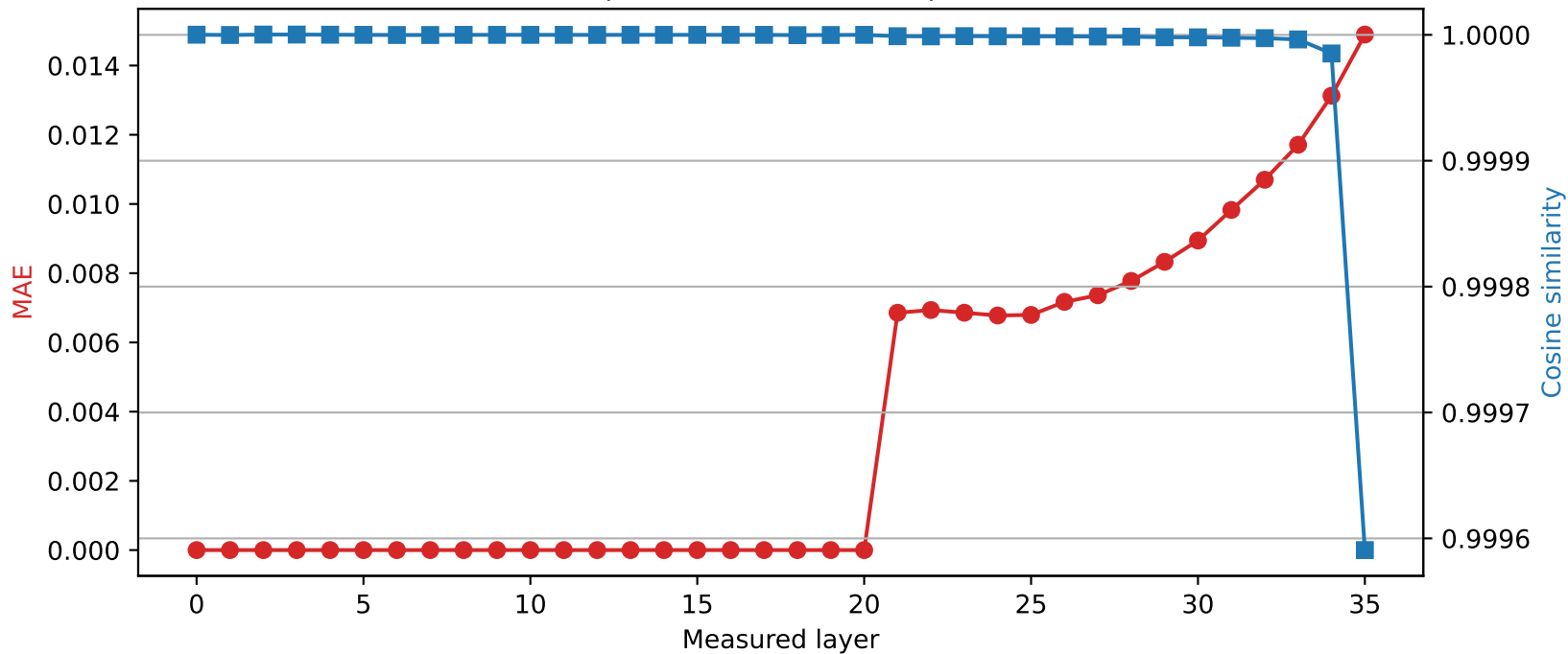
SmolLM3-3B | Quantized layer 20 | float64 → int8
