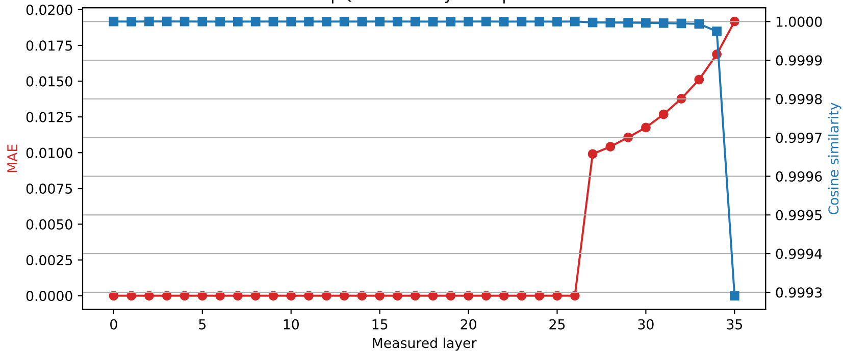
SmolLM3-3B | Quantized layer 26 | float64 → int8
