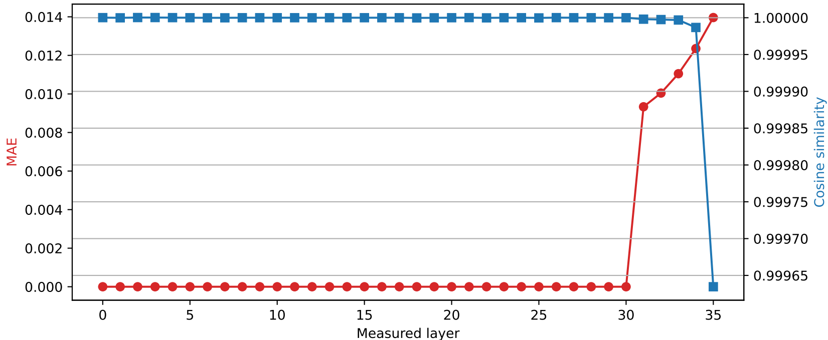
SmolLM3-3B | Quantized layer 30 | float64 → int8
