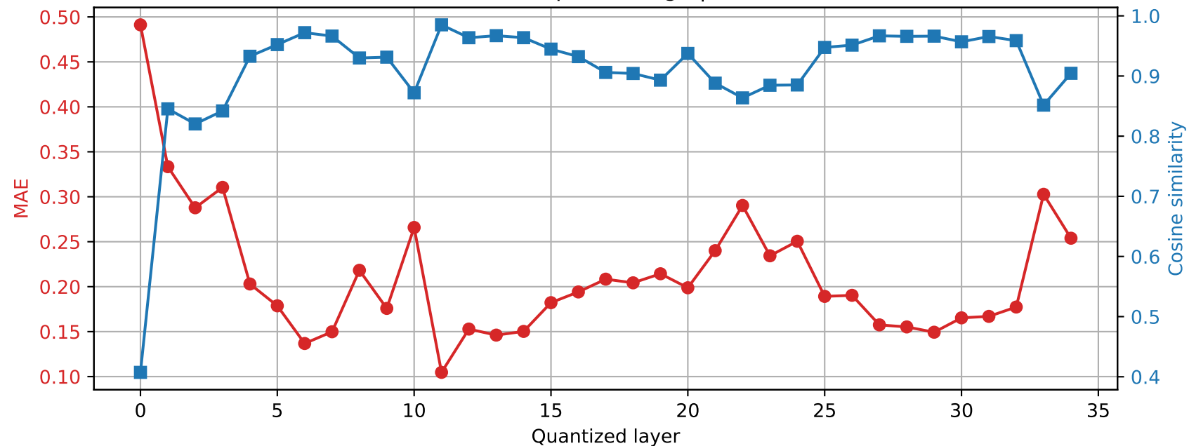
SmolLM3-3B | Prompt 0 Final RMSNorm output damage | float64 \rightarrow int4
