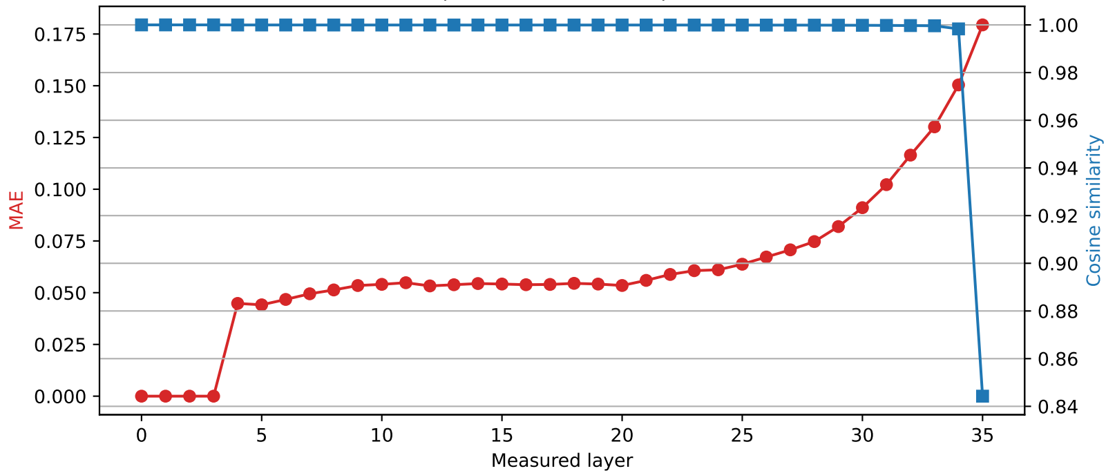
SmolLM3-3B | Quantized layer 3 | float64 → int4
