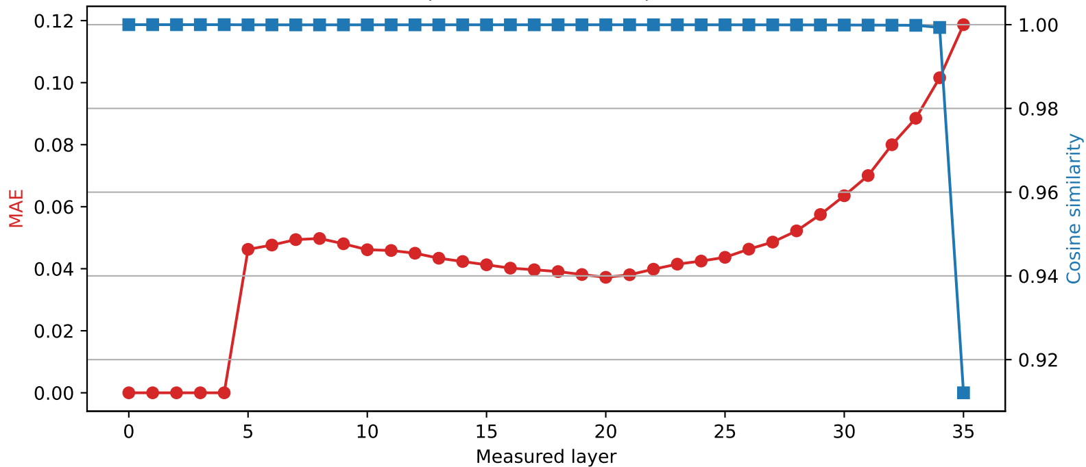
SmolLM3-3B | Quantized layer 4 | float64 → int4
